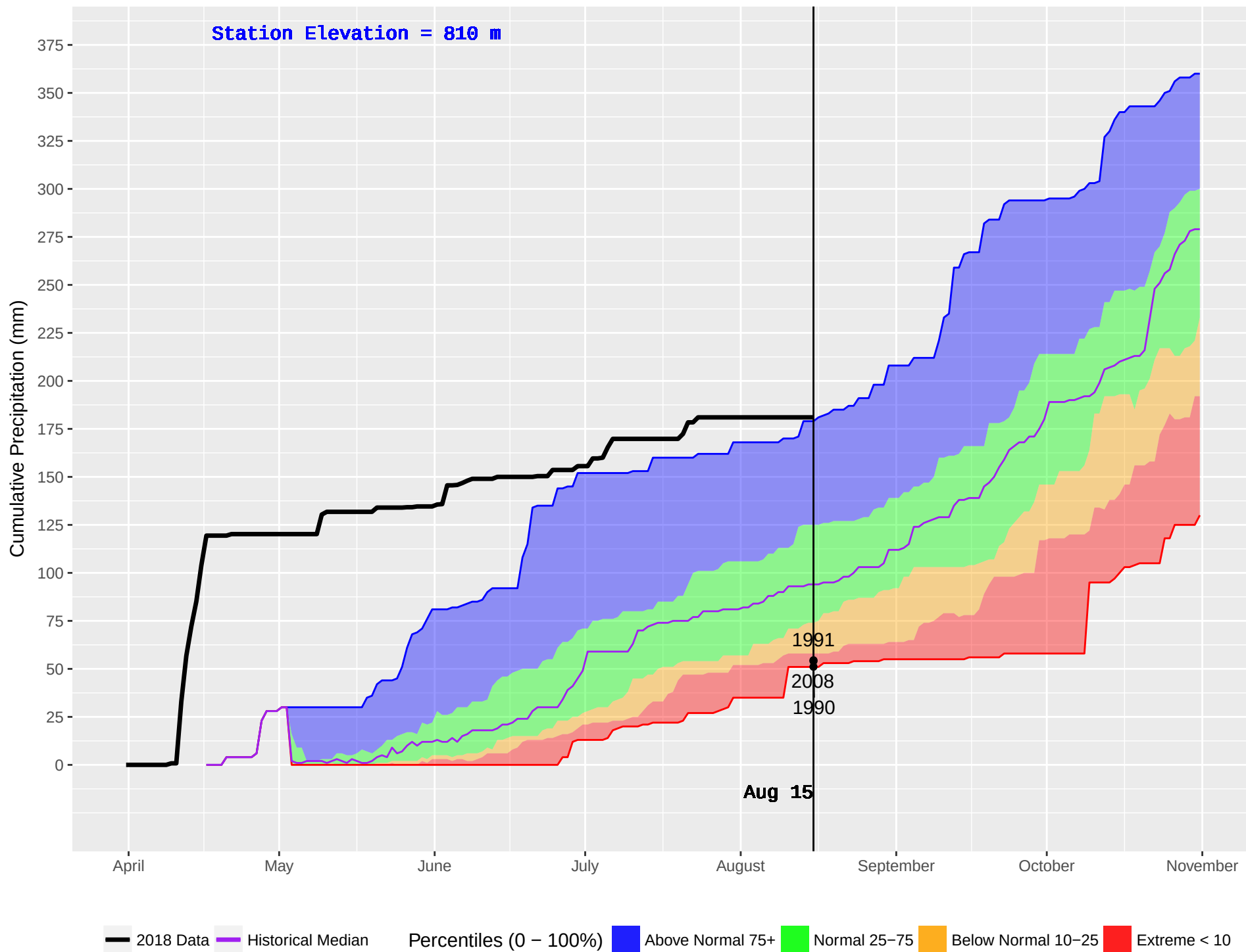
MCBRIDE LAKE (180) : Historical (1990–2016) and Current (2018) Daily Cumulative Precipitation
