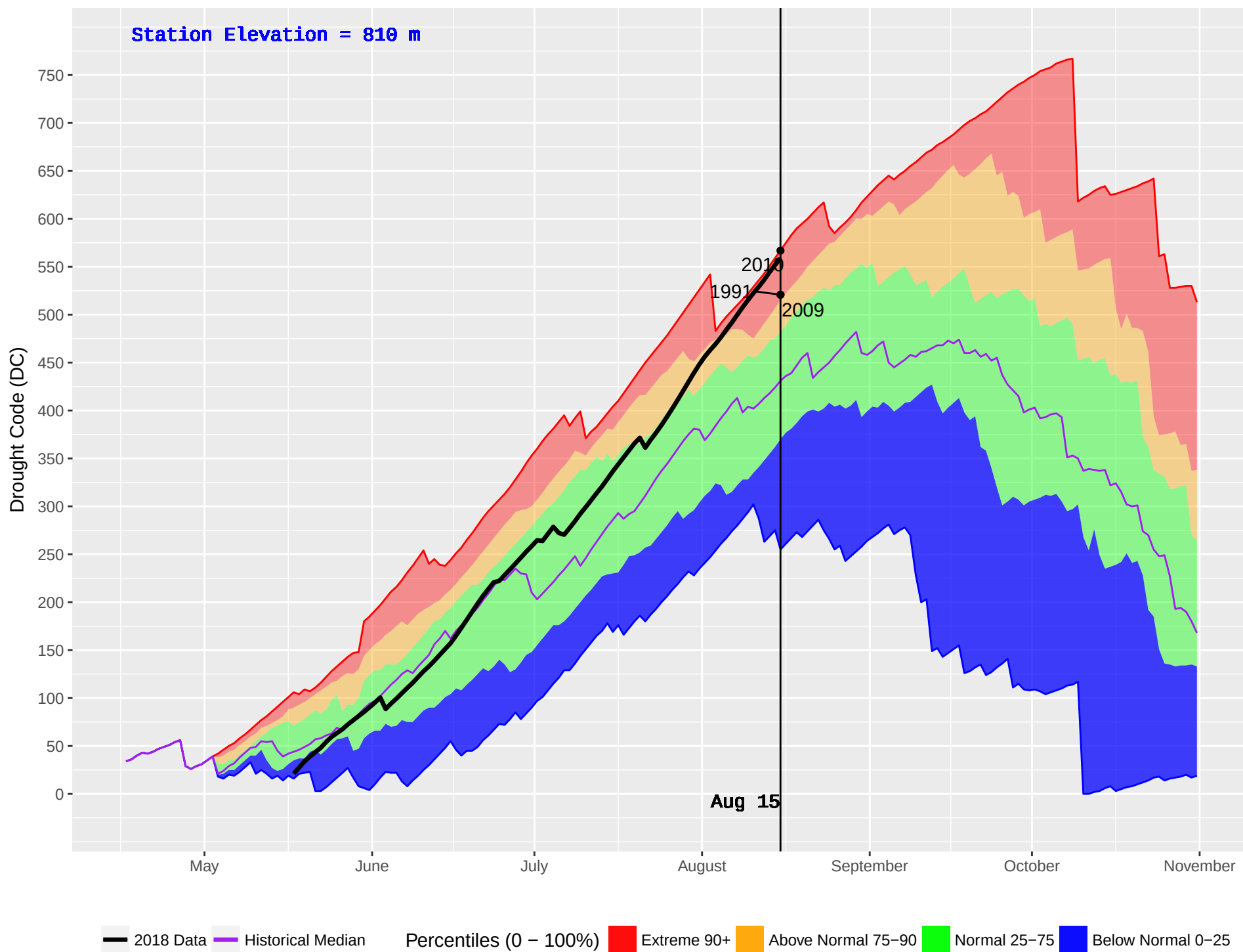
MCBRIDE LAKE (180) : Historical (1990–2016) and Current (2018) Daily Drought Code (DC)
